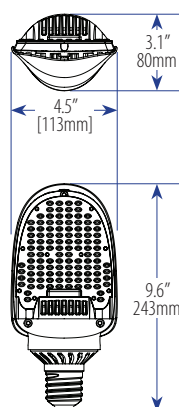
BOTTOM VIEW
